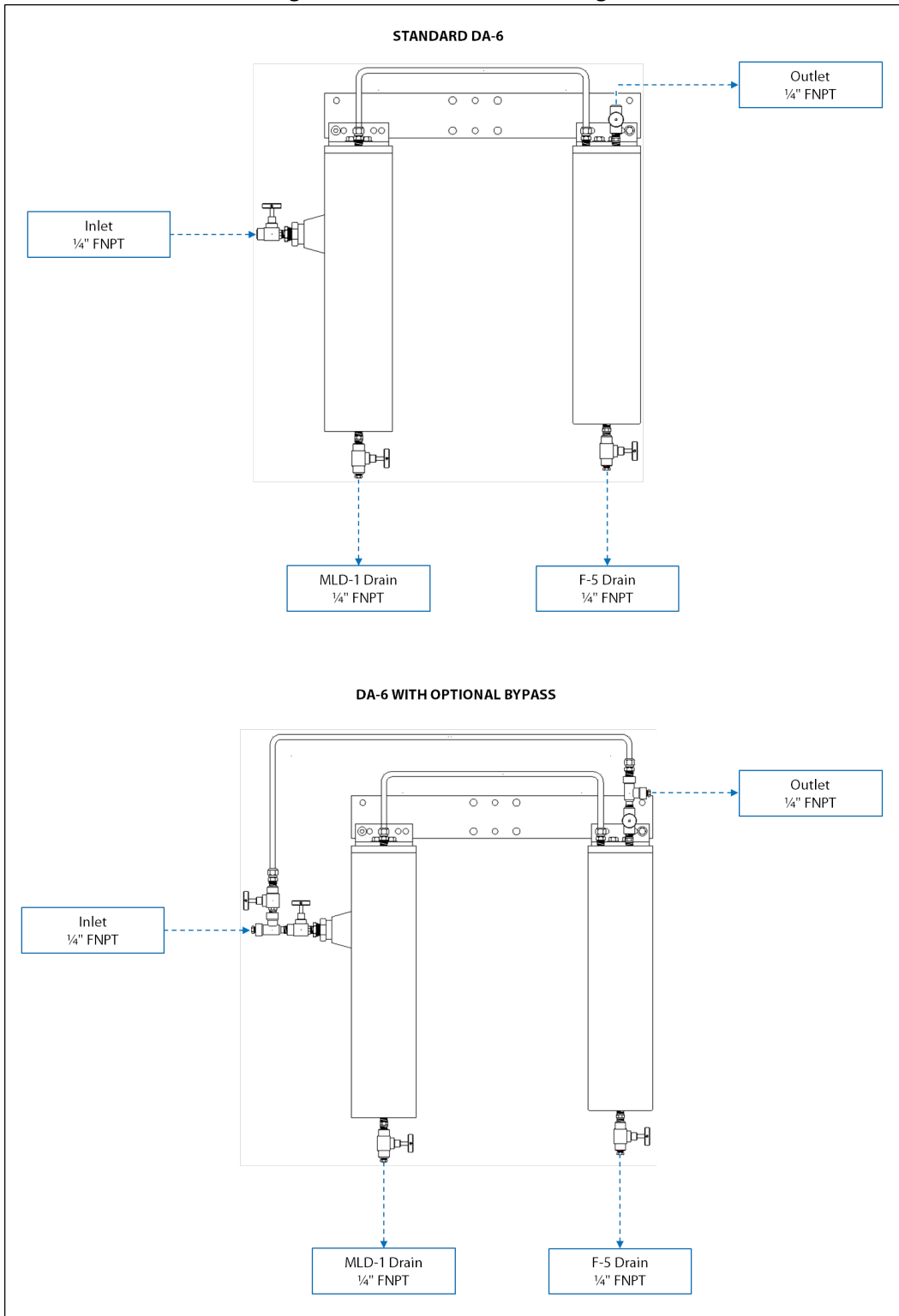
Figure 1: DA-6 Connections Diagram
