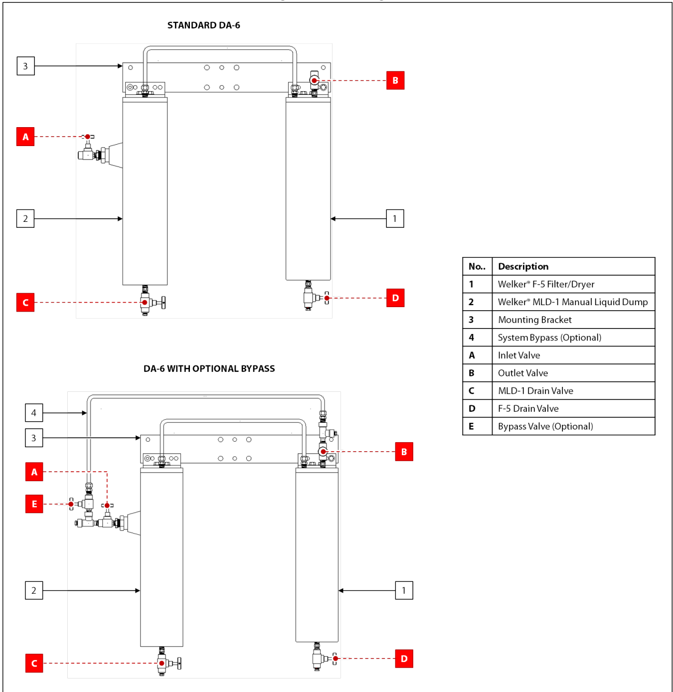
Figure 2: DA-6 Diagram
